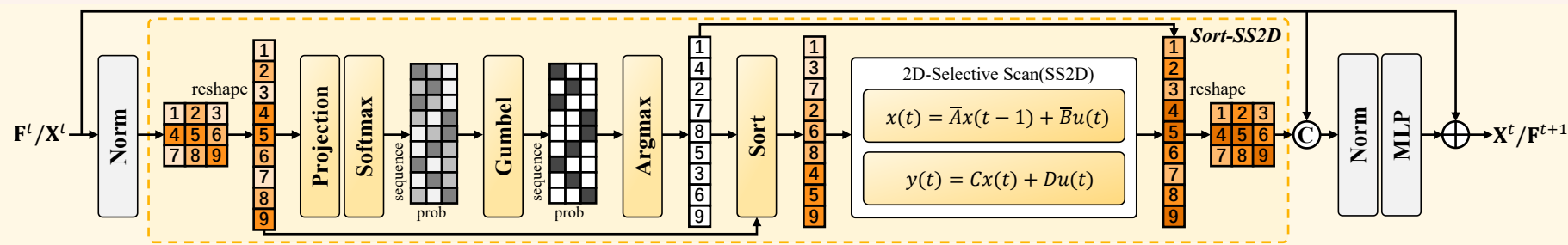
(c) Feature Refinement Module (FRM)
