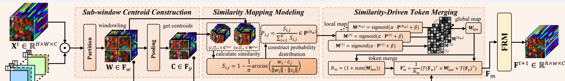
(b) Spatial Semantic-aware Merging Module (S2M)
